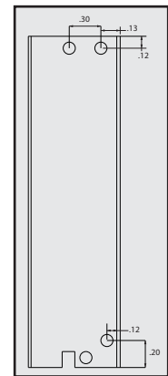
Locations of LED holes on standard AMC panels
